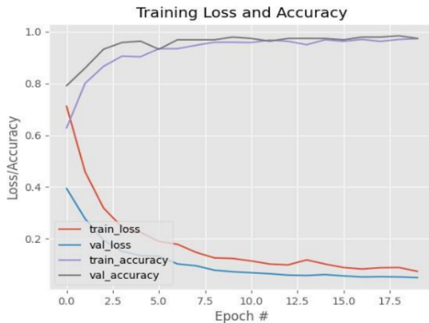
Figure 6. Training process results
