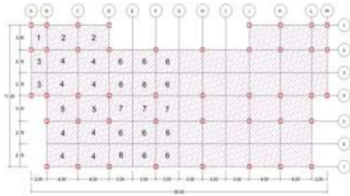
Gambar 3 Denah plat atap
