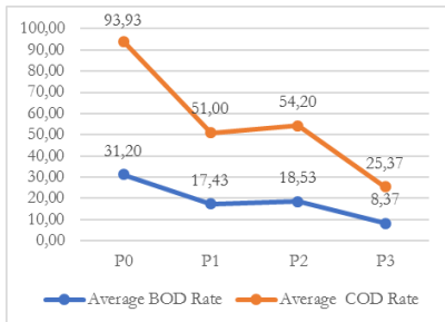
Figure 1. Decrease in BOD and COD levels on day 6
