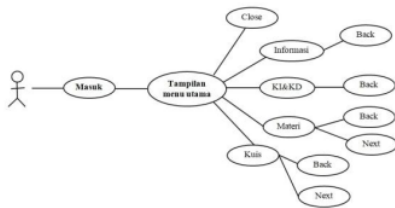
Gambar 1. Use case diagram
