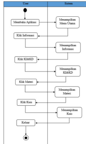
Gambar 2. Activity diagram
