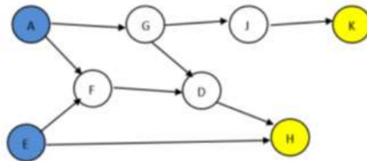
Gambar 1. Ilustrasi proses forward chaining
