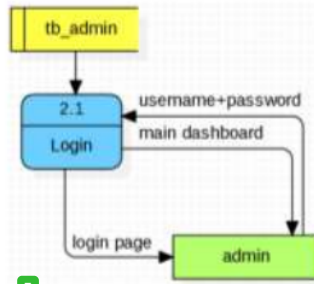
Gambar 8. DFD Level 1 Proses 2.0 Login
