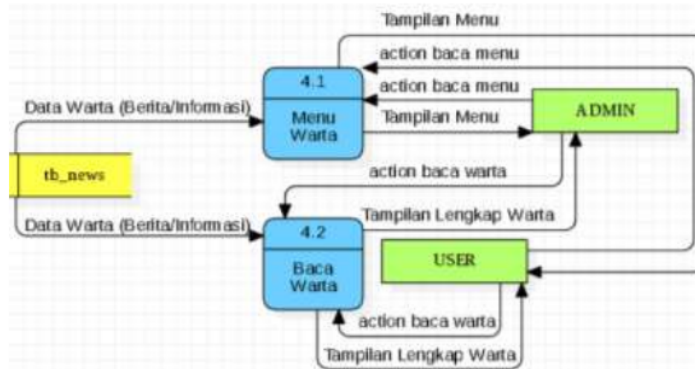
Gambar 10. DFD Level 1 Proses 3.0 Baca warta
