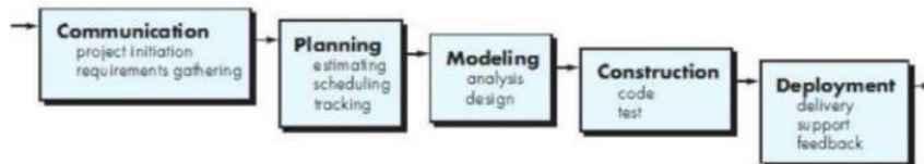
Gambar 2. Metode Waterfall [16]
