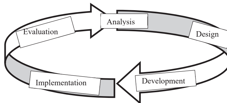
FIGURE 1. ADDIE model
