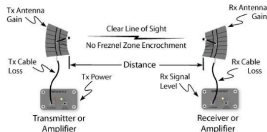
Gambar 1. Link Budget [5]
