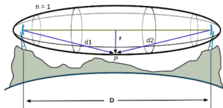
Gambar 2. Fresnel Zone [3]
