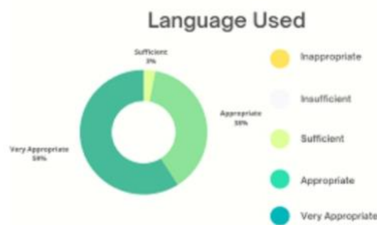
Figure 4: Language Used.
