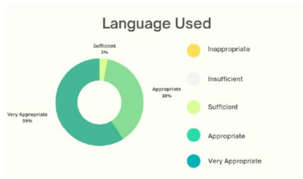
Figure 4. Language Used
