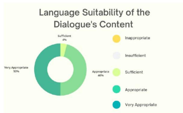
Figure 5. Dialogue's Content
