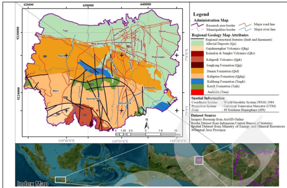
Figure 1. Geological Map of Semarang Area (modified from Thanden et al. , 1949).
