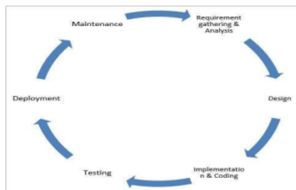
Gambar 1. Tahapan SDLC.
