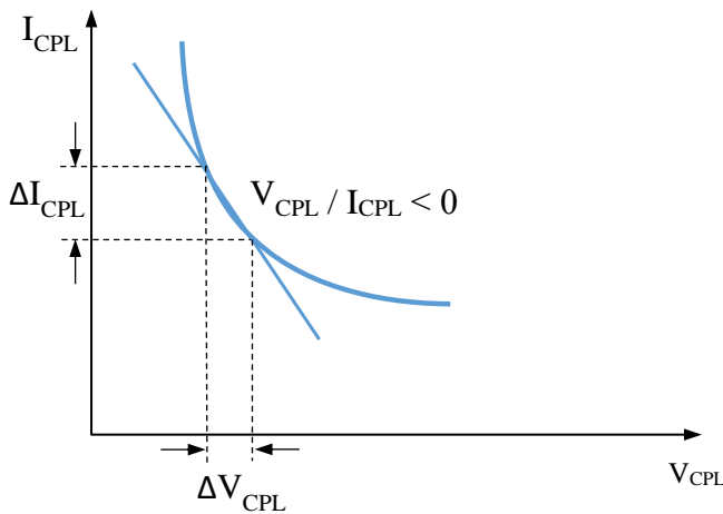
Fig. 1 CPL negative resistance.
