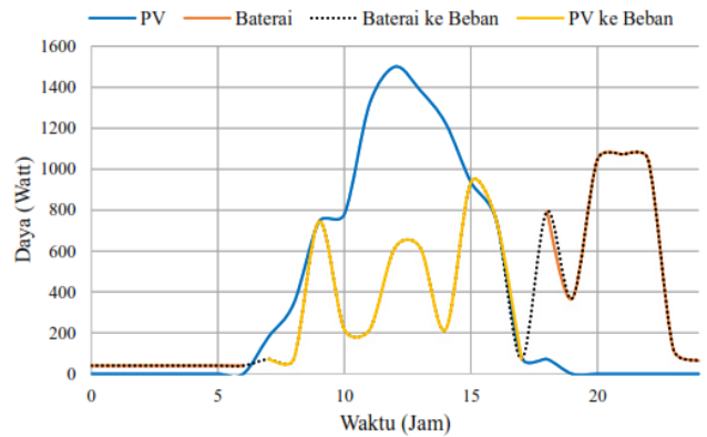
Fig. 10 Load and source graph of the four residential microgrid.
