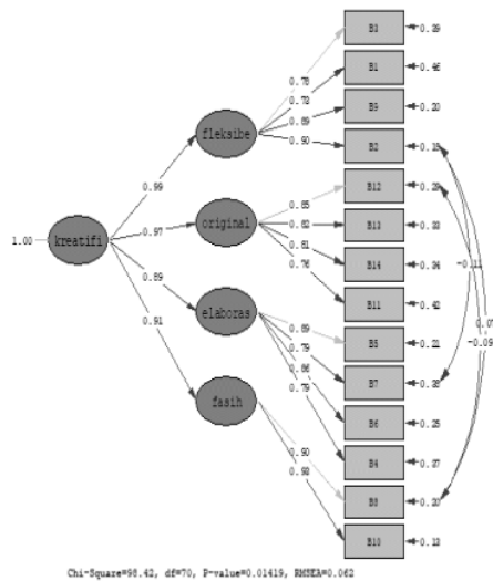
Gambar 2. Standardize solution second order CFA instrumen kreativitas
