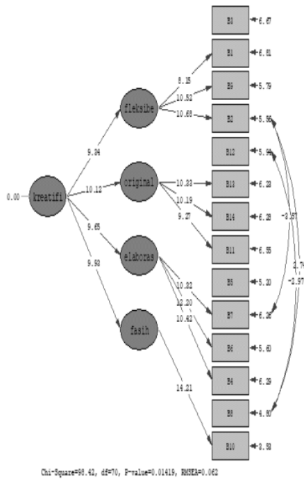
Gambar 1. T-value second order CFA instrumen kreativitas
