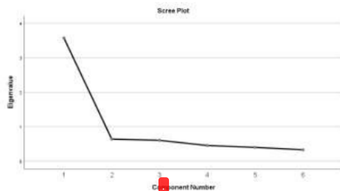
Gambar 1. Scree Plot
