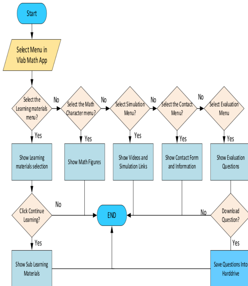
Figure 5. Scenario Use of V-Lab Math Application
