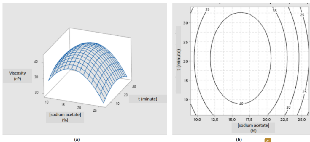
Figure 3. Response surface (a) and contour curve (b) for viscosity of cross-linked canna starch
