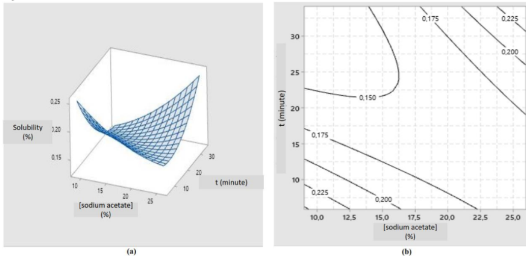
Figure 5. Response surface (a) and contour curve (b) for solubility of cross-linked canna starch
