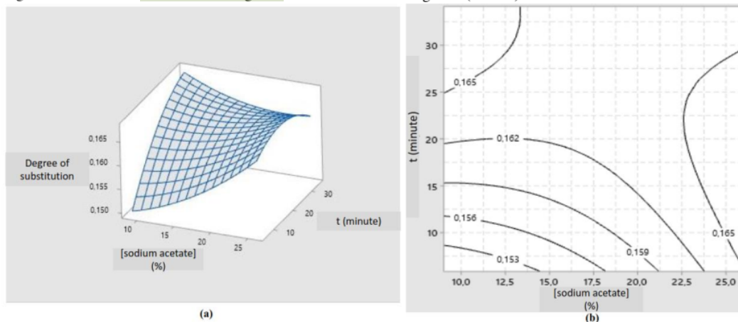
Figure 1. Response surface (a) and contour curve (b) for the degrees of substitution of cross-linked canna starch
