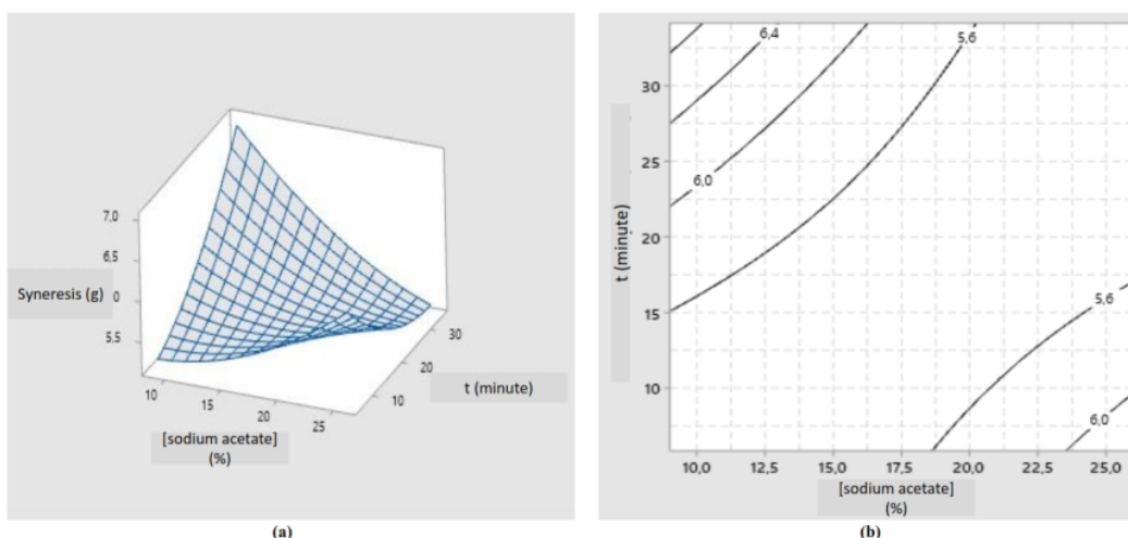
Figure 6. Response surface (a) and contour curve (b) for syneresis of cross-linked canna starch
