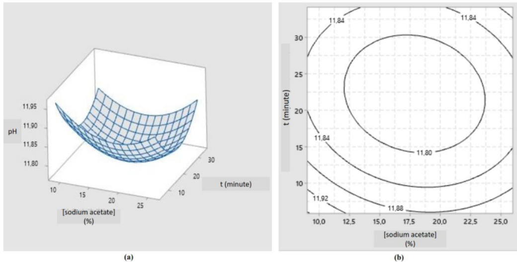
Figure 7. Response surface (a) and contour curve (b) for pH of cross-linked canna starch
