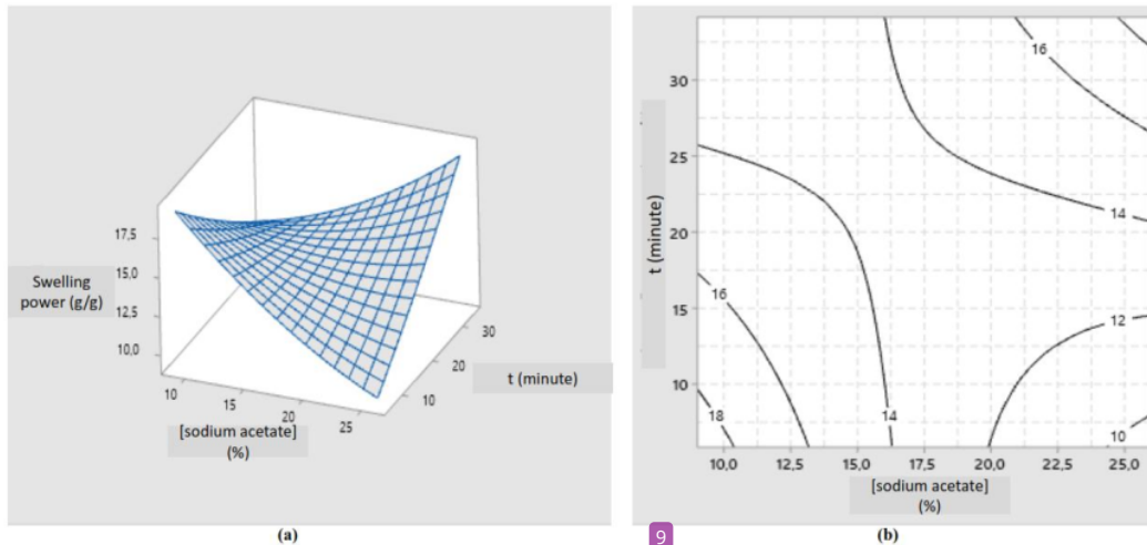
Figure 4. Response surface (a) and contour curve (b) for swelling power of cross-linked canna starch
