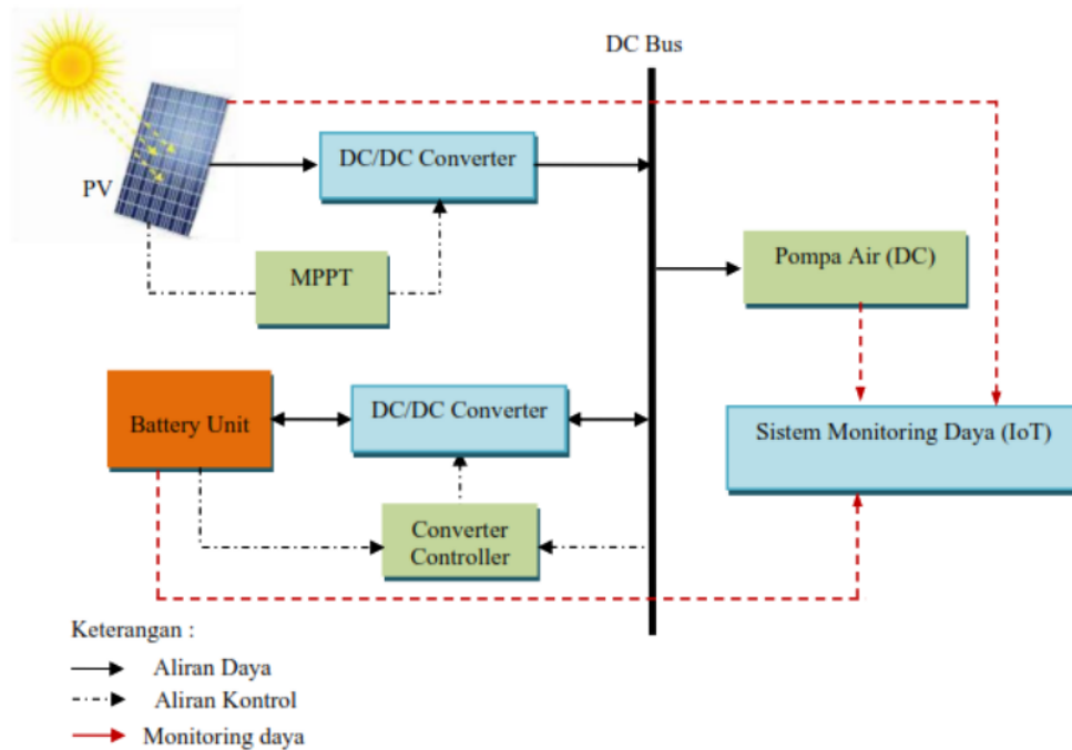
Gambar 2. Pompa air tenaga surya dilengkapi system monitoring.
